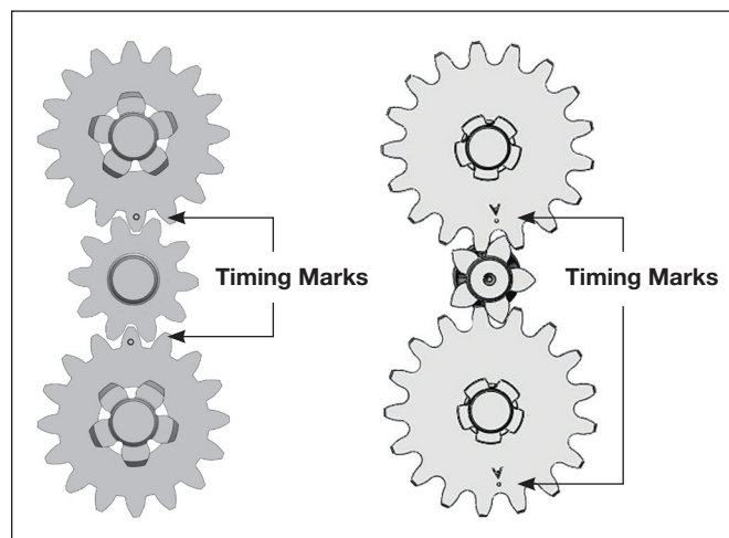
Figure 10 - Gear Timing (0.75 and 1.5 Tonne)
