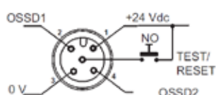
RX: M12 5-POLE CONNECTOR
