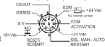
RX: M12 8-POLE CONNECTOR
