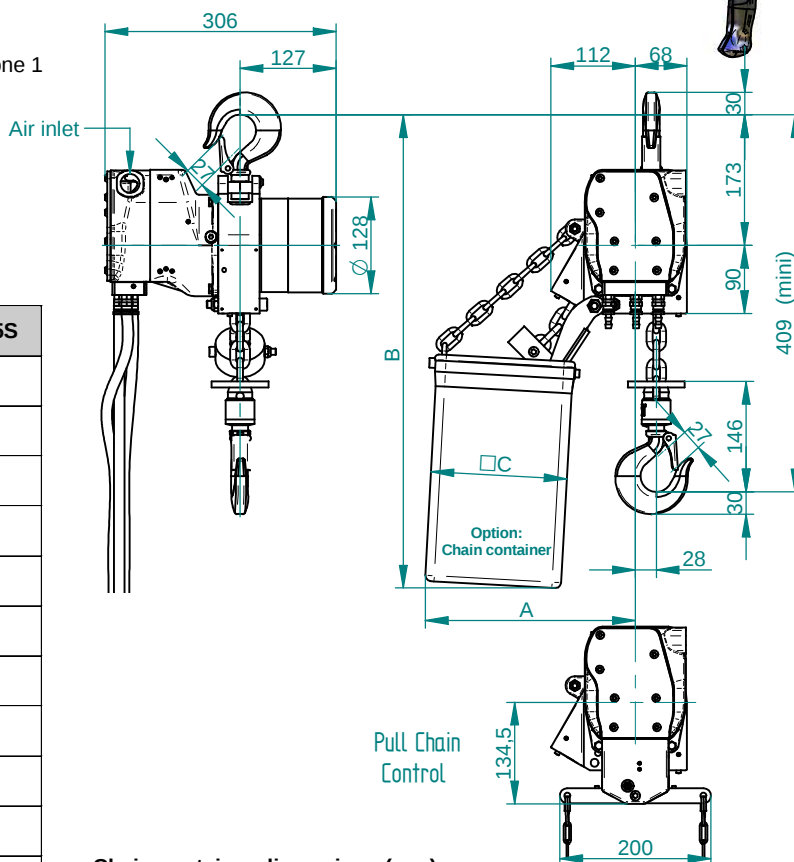
Chain container dimensions (mm)
