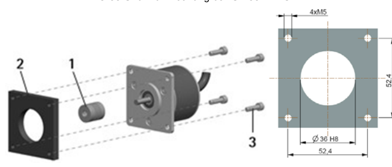
ENC-58-S10 with mounting bell ST-58-FLNG
