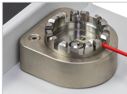
▲ The standard adjustable wire terminal fixture accommodates wire diameter sizes up to AWG 3 (0.25 in [6.3 mm]).
