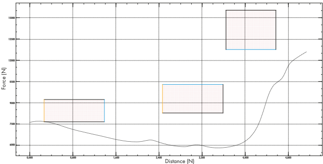
Example NOK process Material to be joined too thin due to missing component
