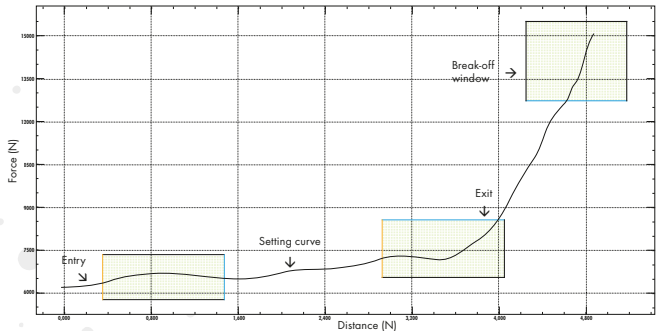
Example OK process Window entry and exit at customer-defined positions
