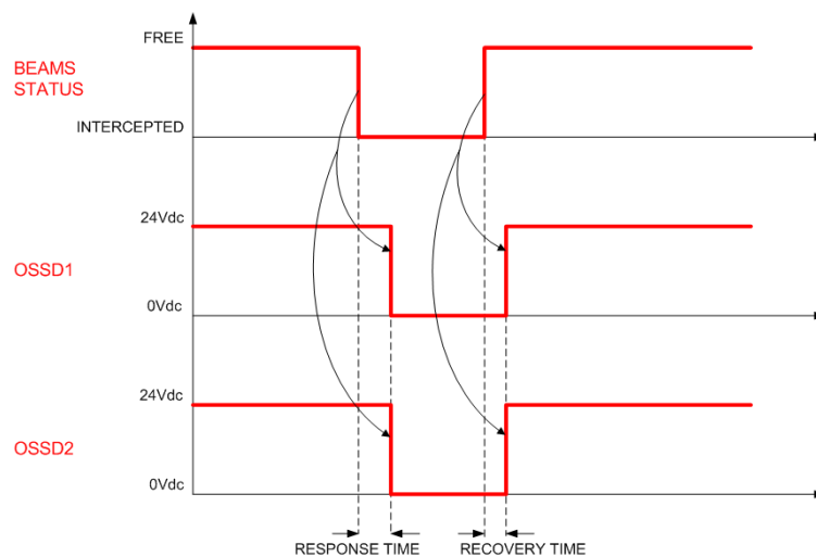
Fig. 56 – PNP timings
