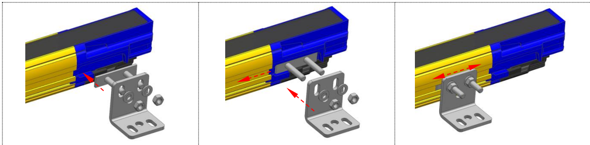
Fig. 17 – Fixed brackets mounting procedure
