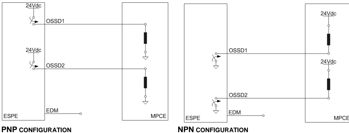
Fig. 37 – EDM connection
