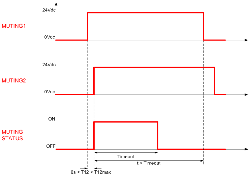
Fig. 45 – Muting timeout
