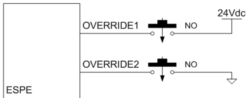
Fig. 48 – Override connection
