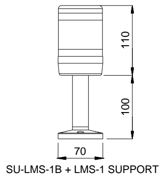
SU-LMS-1B + LMS-1 SUPPORT
