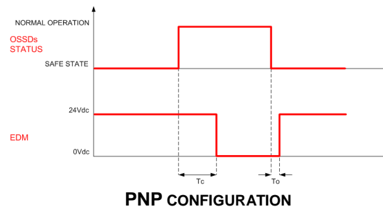
PNP CONFIGURATION
