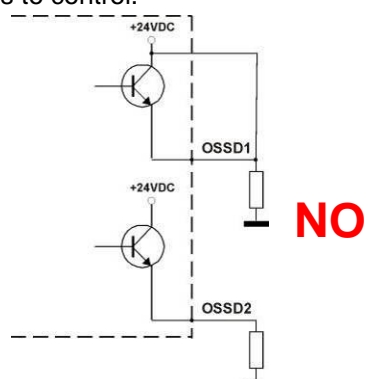
Fig. 22 – Incorrect connection of the load (I)
