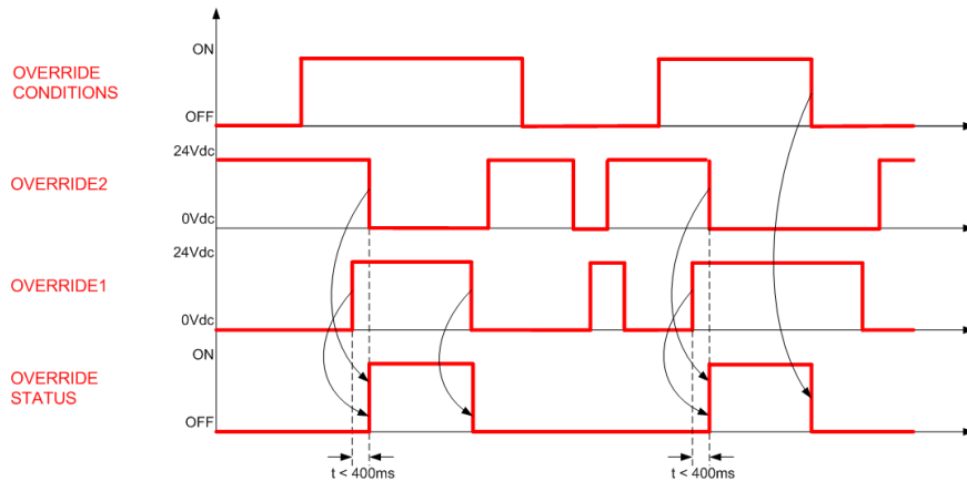
Fig. 49 – Override timings (level trigger)
