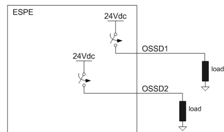
FIG. 55 – PNP CONNECTION
