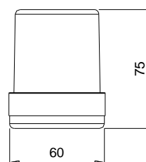
LMS-2 LAMP
