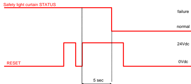
Fig. 35 – Reset timings
