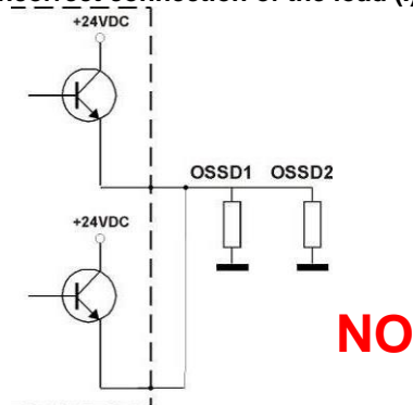
Fig. 24 – Incorrect connection of the load (III)
