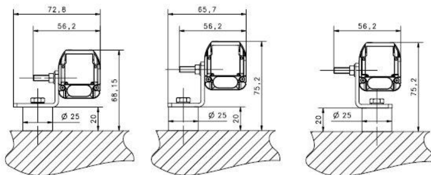
Angled fixing bracket + Antivibration support
