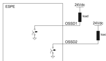
FIG. 57 – NPN CONNECTION
