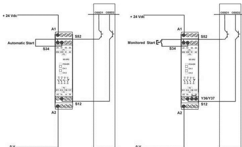
Connection to safety relay
