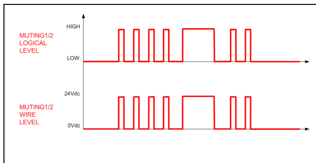
Fig. 46 – Muting filter disabled
