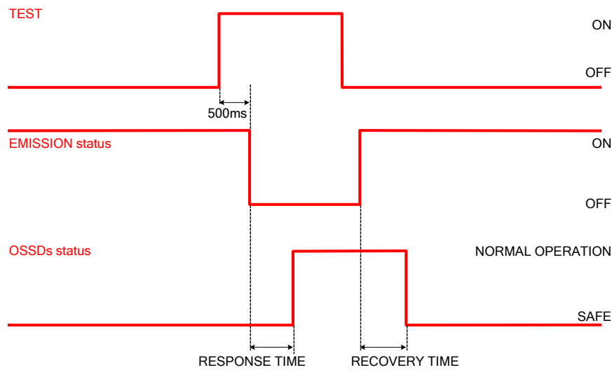
Fig. 34 – Test timings
