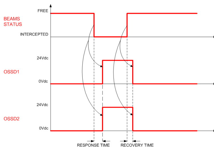
Fig. 58 – NPN timings
