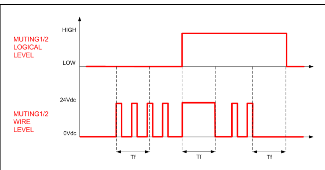
Fig. 47 – Muting filter enabled
