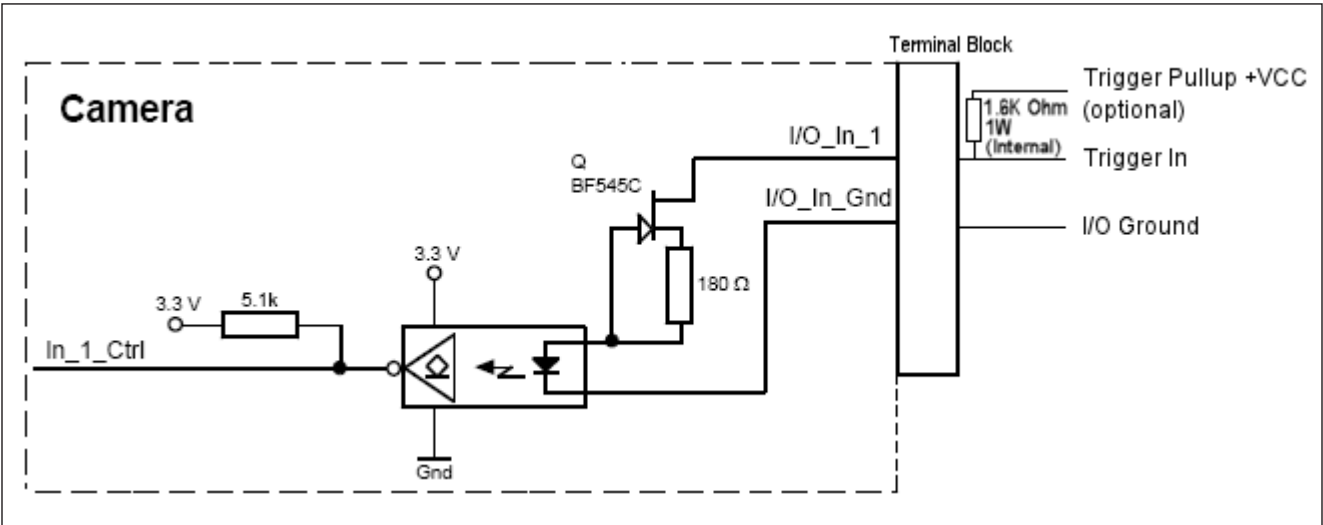
M2xx and M3xx Strobe Trigger Out Circuit
