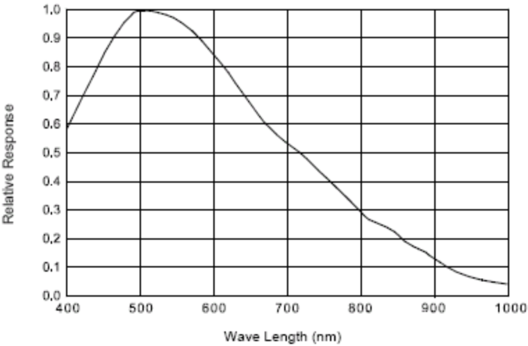
M210 Spectral Response (excludes lens and light source characteristics)
