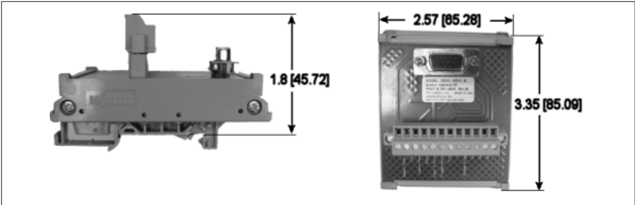
661-0400 Terminal Block Dimensions
