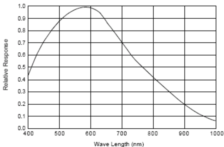
M250 Spectral Response (excludes lens and light source characteristics)
