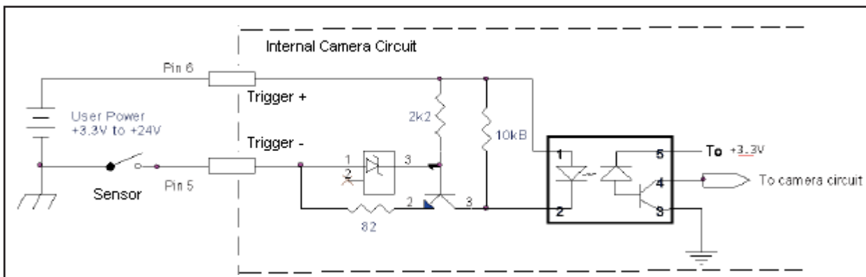
JAI Camera Trigger Input Circuit (sinking)
