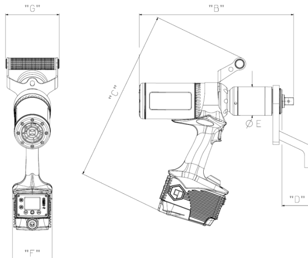
FIGURE 57 – Tool Dimensions
